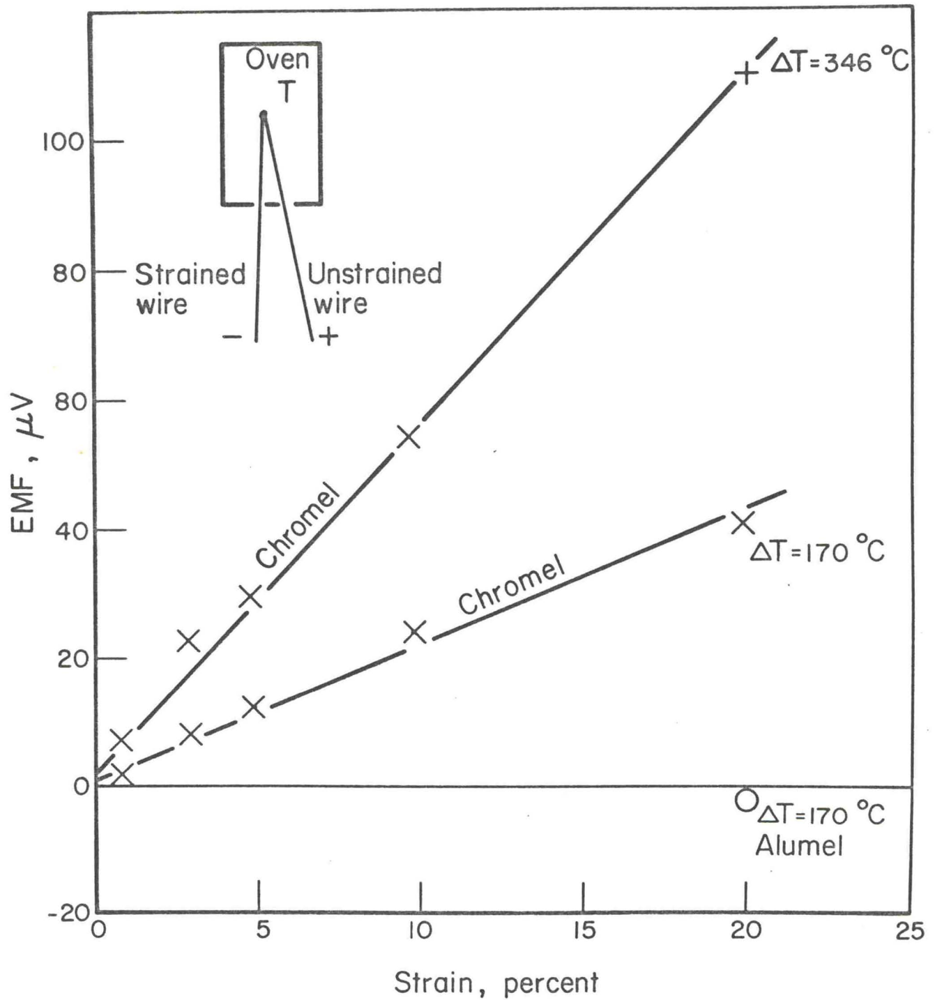
EFFECT OF PERMANANT STRAIN OF THERMOCOUPLE WIRE
